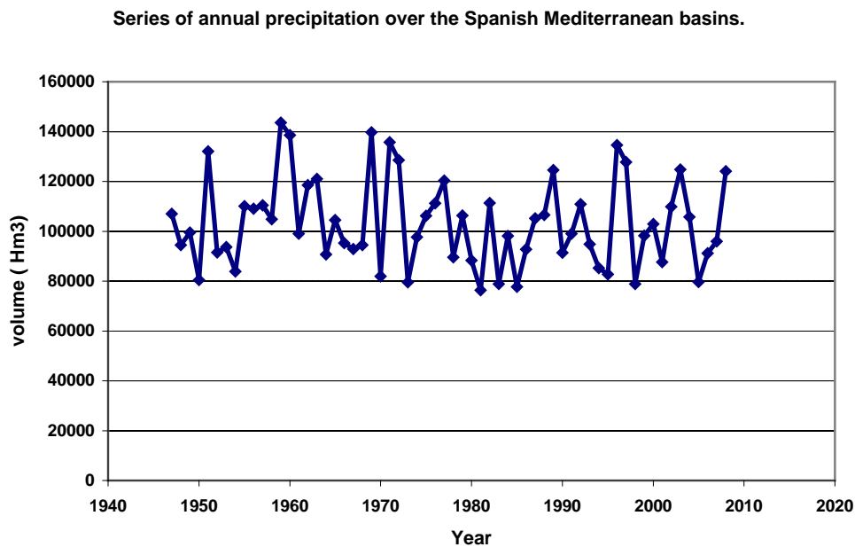
Figure 3. Precipitation variability in Spain; series of annual precipitation over the Mediterranean basins (period: 1947-2008).
